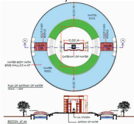
Plan and Site Section of the Proposed work
