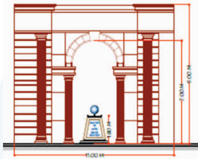
Elevation of the Proposed work
